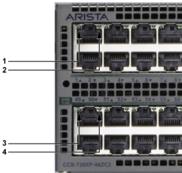
Figure 8: Port LEDs
