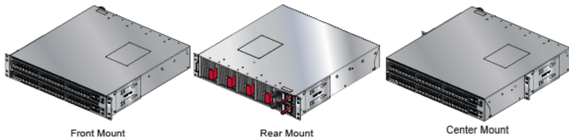
Figure 2: Improper Bracket Mount Examples for Two-Post Rack Mount
