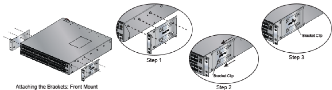
Figure 3: Attaching the Mounting Brackets to the Switch Chassis
