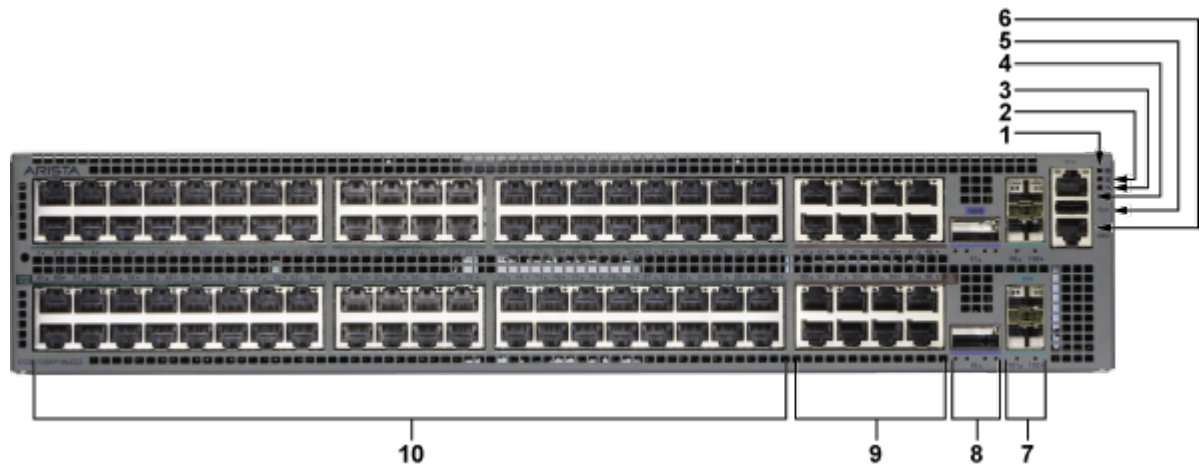
Figure 12: CCS-720XP-96ZC2
