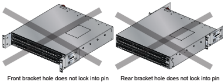
Figure 2: Improper Bracket Mount Examples for Two-Post Rack Mount
